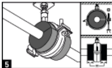
Push insulation into the bracket. Caution: Make sure the rigid foam is positioned correctly.
