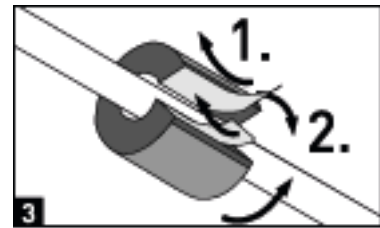
Assemble insulation 1. Peel off foil 2. Press on contact area
